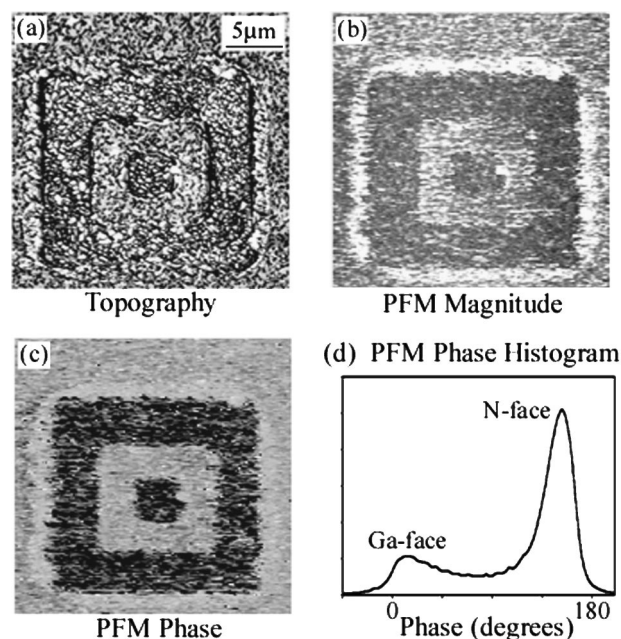
FIG. 1. (a) Topographic, (b) PFM magnitude, and (c) PFM phase images of a GaN-based lateral polarity heterostructure. The innermost 5 \times 5 \mu\text{m}^2 square is the Ga-face region. The N-face region has a higher piezoresponse magnitude as indicated by contrast, and there is a sharp contrast difference in the piezoresponse phase image, demonstrating inversions in film polarity. (d) Histogram of the PFM phase image (c). The magnitudes of the Ga- and N-face peaks correspond to the relative areas of each region.
